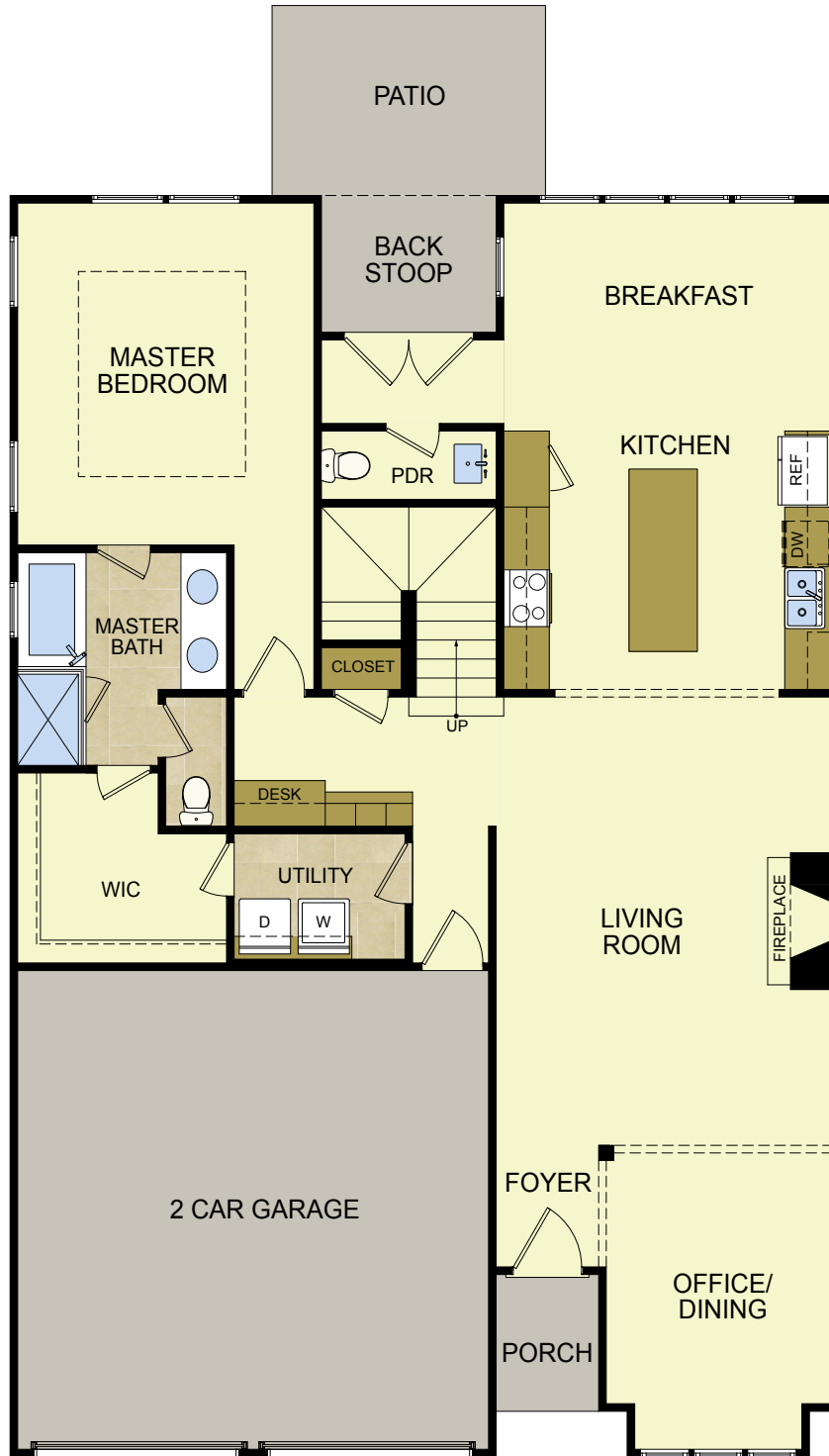
FIRST FLOOR
