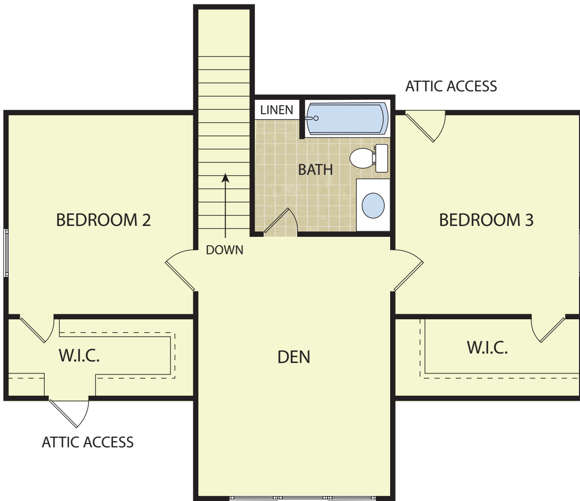
SECOND FLOOR
