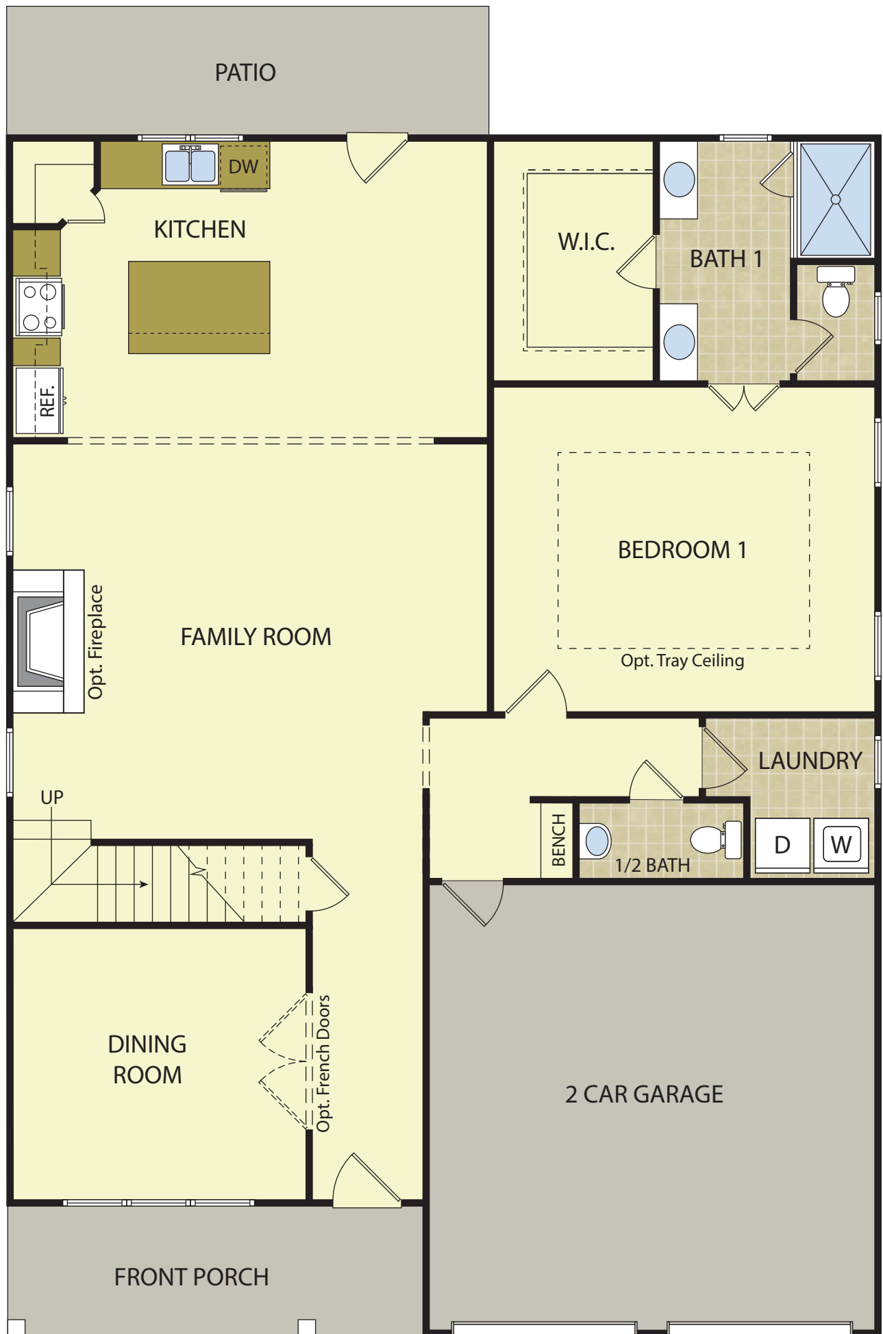
FIRST FLOOR
